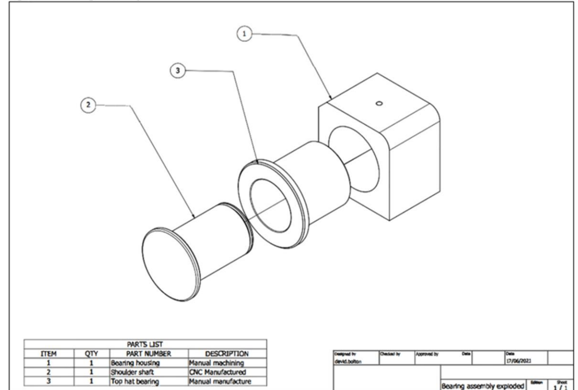
Figure 1 – Bearing assembly
